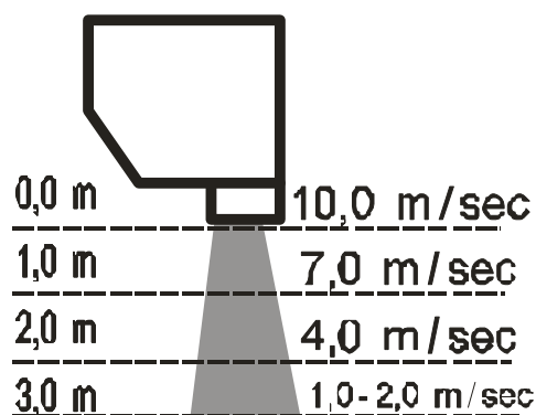
AIR VELOCITY DISTRIBUTION CHART
