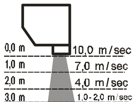
AIR VELOCITY DISTRIBUTION CHART
